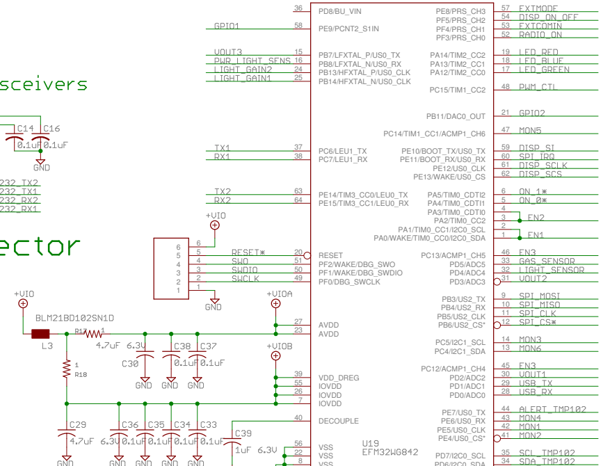
EFM Microcontroller
